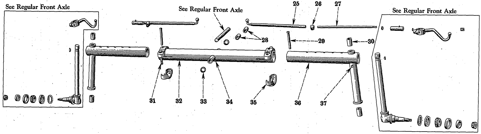
ADJUSTABLE FRONT AXLE ATTACHMENT (Special)
